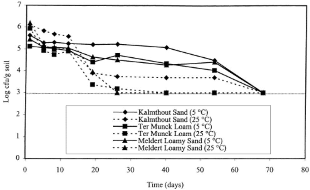
Fig. 1. Survival of E. coli in three soil textures at two incubation temperatures.
